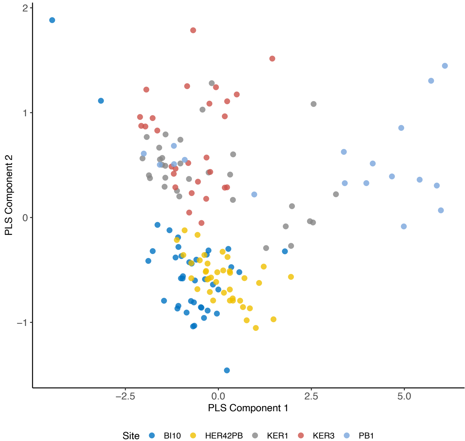
PLSR Score Plot (Training Data) - Ti, Ca, Sr, Zr
